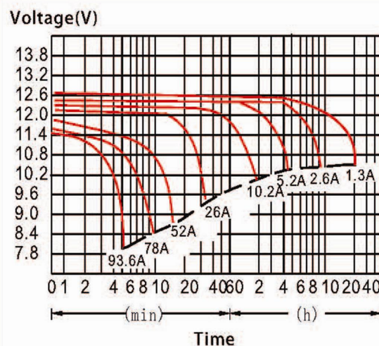
Constant Current(Amp) and Constant Power(Watt) Discharge Table at 25℃(77℉)
